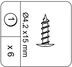
SCREW TCS1065
